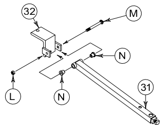
Detail "A" Parts Breakdown of Part # 705009
