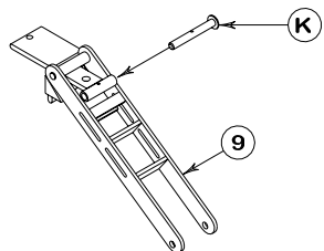
Detail "A" Parts Breakdown of Part # 705009
