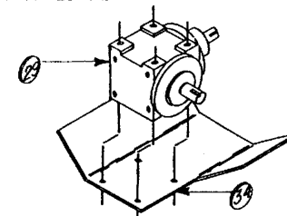
DETAILED VIEW OF PTO GEAR BOX
