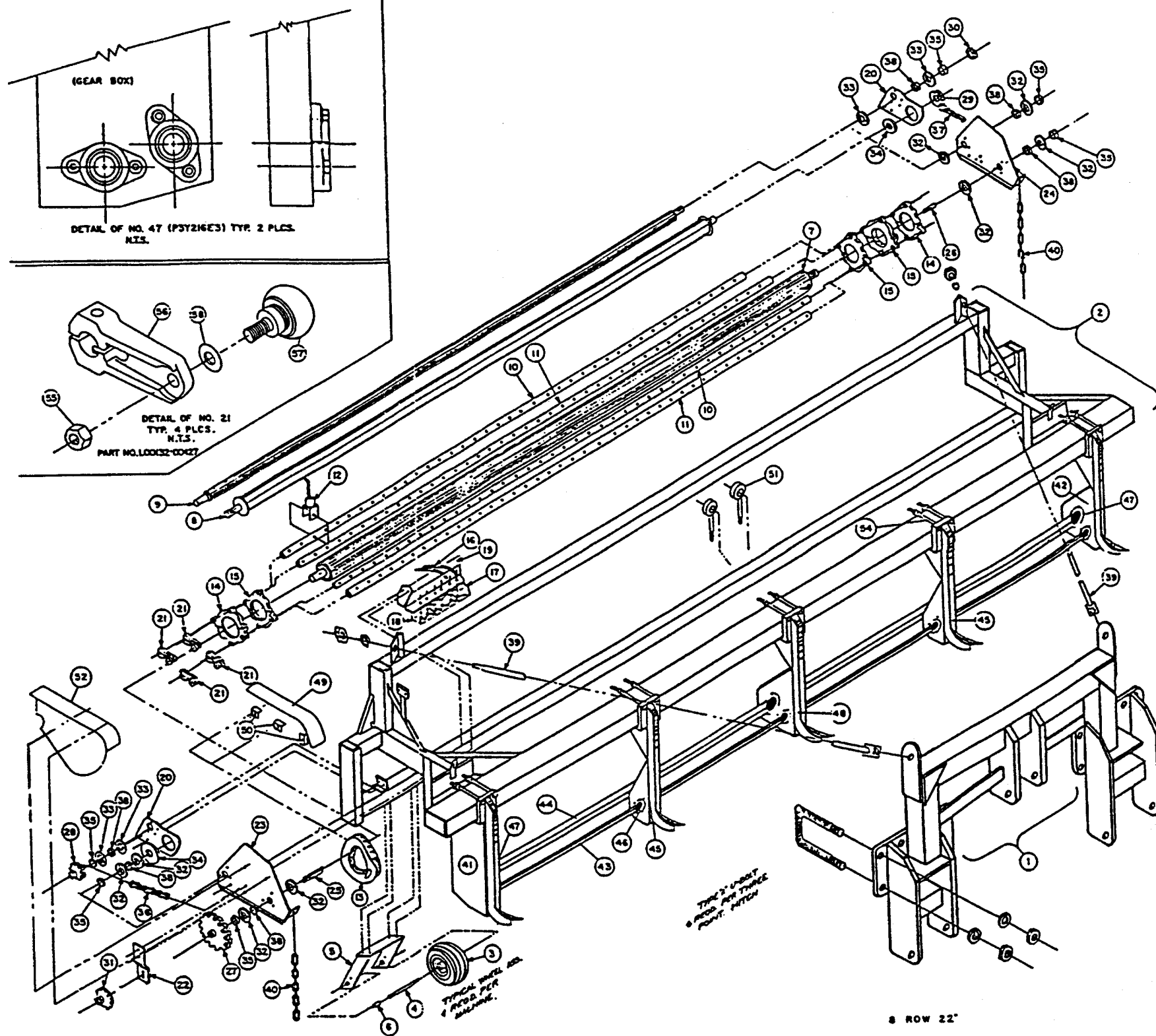
BASIC MACHINE
