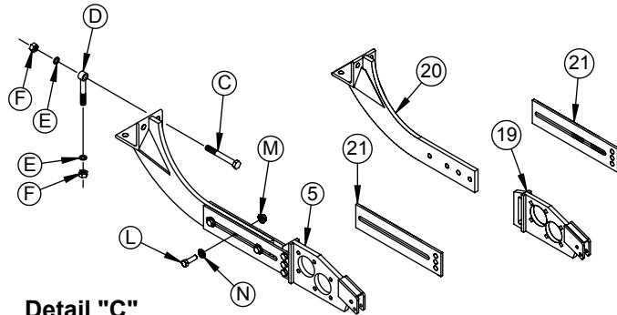
Detail "C"
