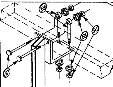
TYPICAL MOUNTING HARDWARE FOR 6x4 TOOL BAR
